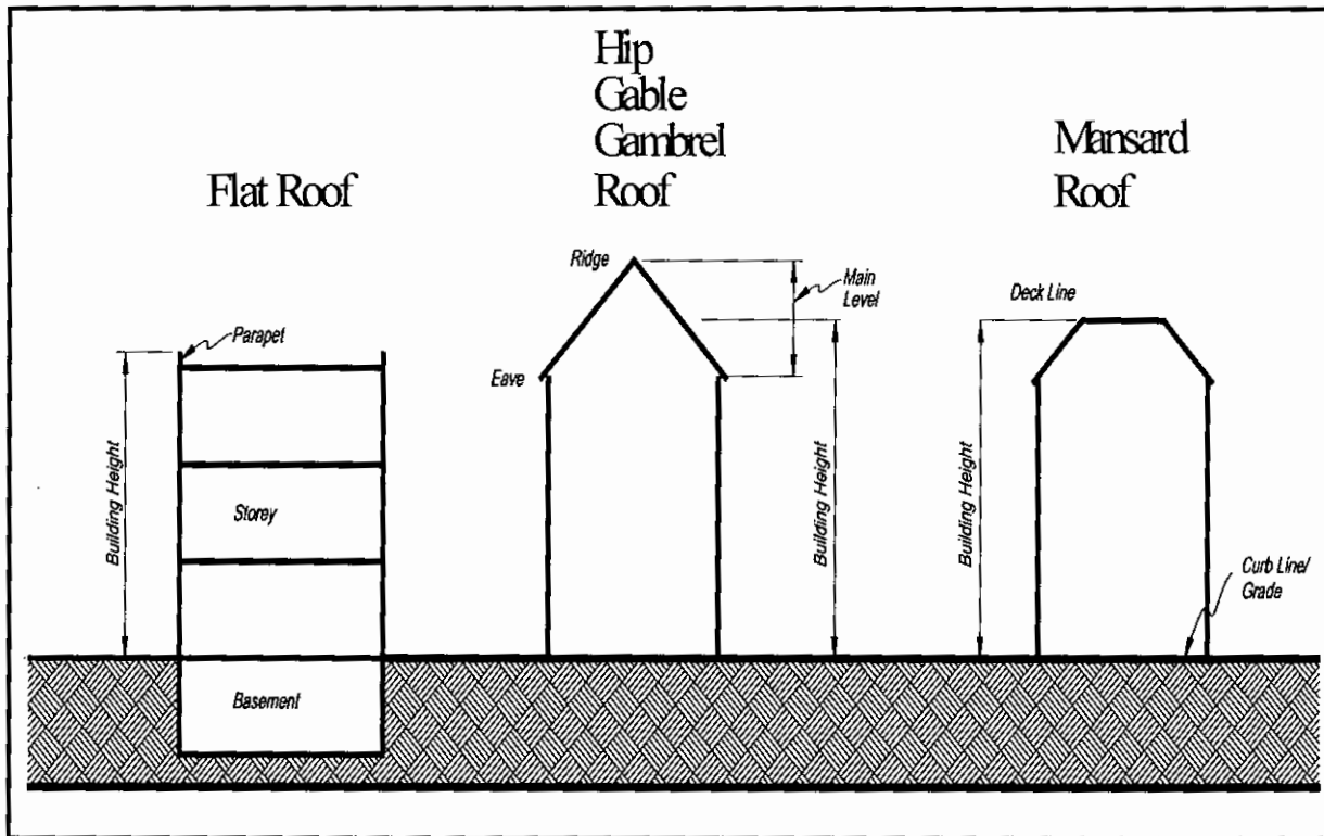
Figure 3. Height of Buildings
